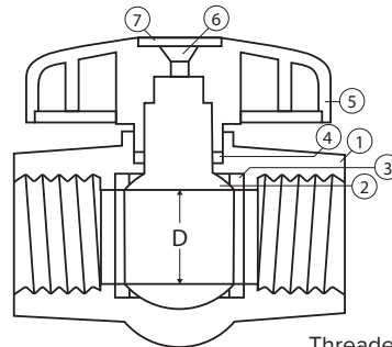
Threaded Connection
