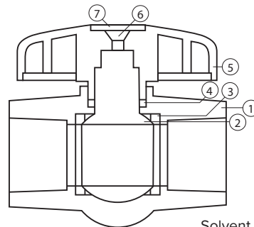
Solvent Connection
