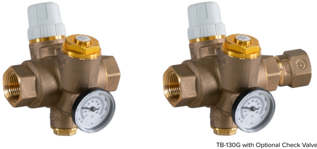
TB-130G with Optional Check Valve
