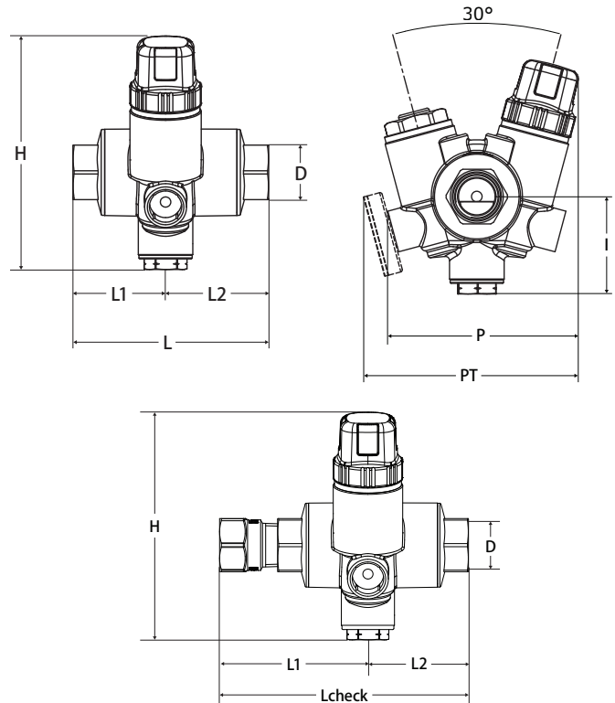
TB-130G with Optional Check Valve
