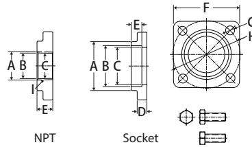
TYPE B (WITHOUT O-RINGS)
