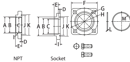
TYPE A (WITH O-RINGS)
